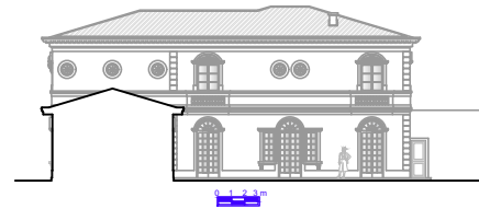
Elevation 03
